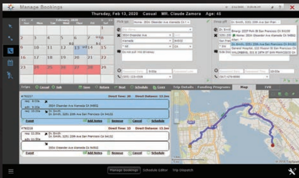
> REAL-TIME SCHEDULING
